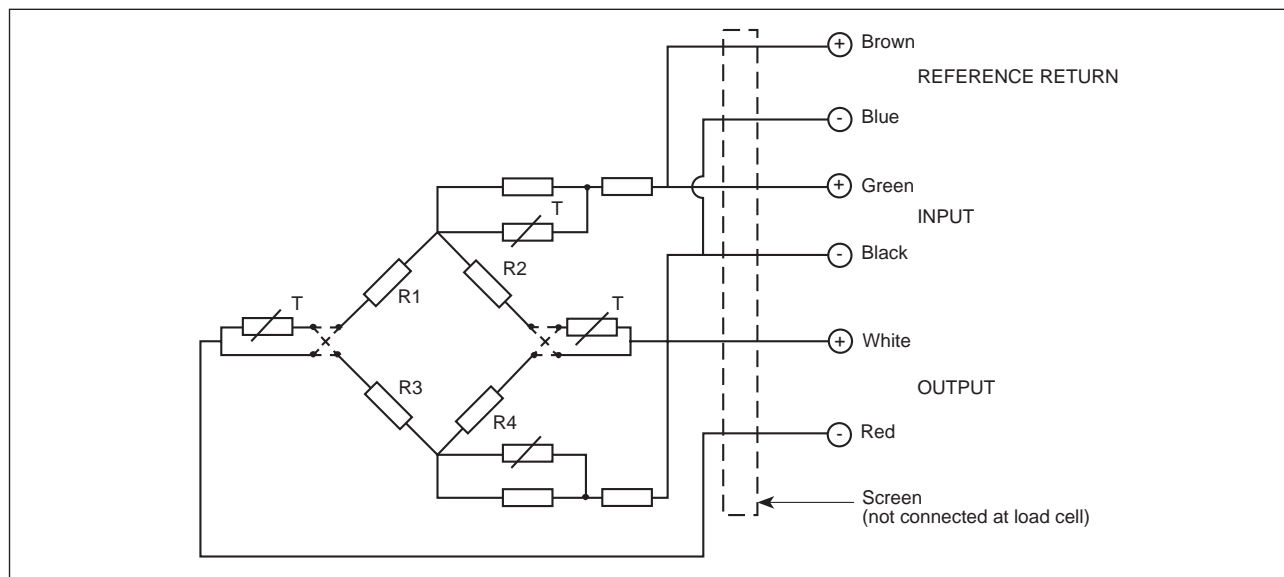
Circuit Diagram.
